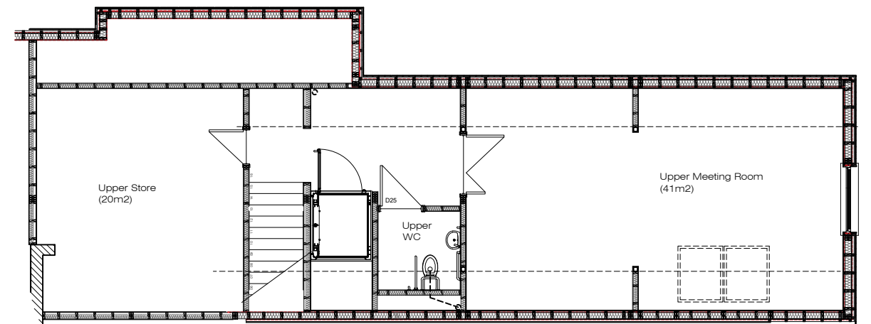
FIRST FLOOR CONSTRUCTION PLAN
